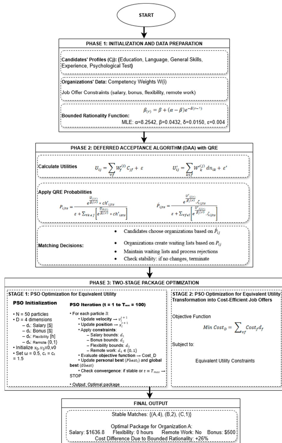
Figure 4. Algorithm Flowchart.
